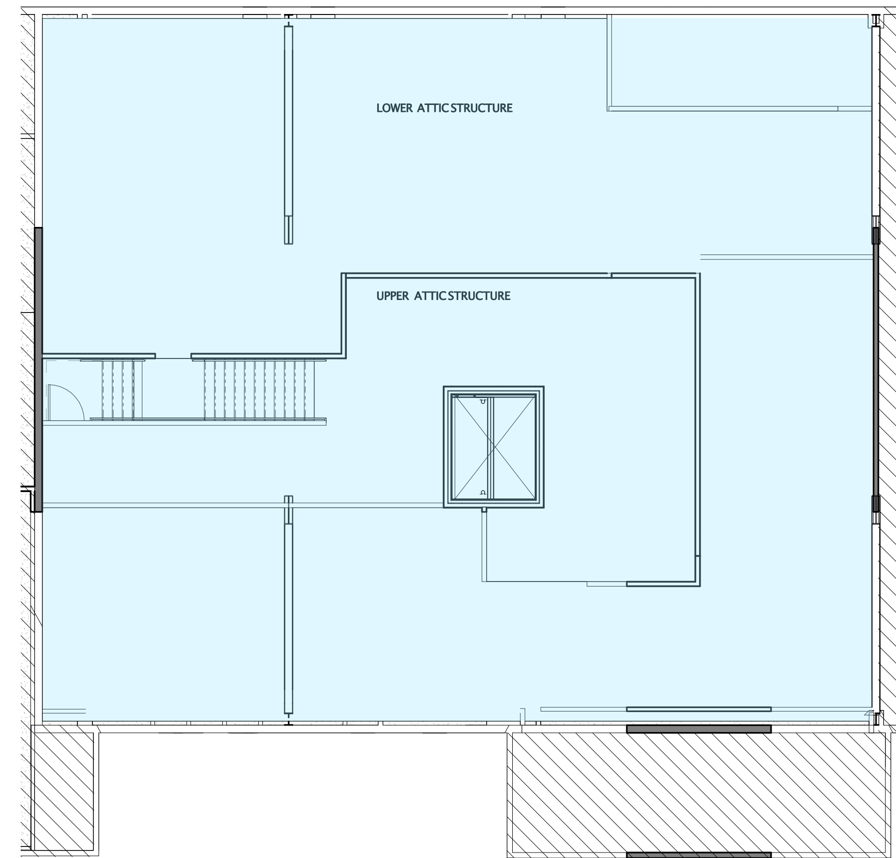
UPPER ATTIC AND LOWER ATTIC FLOOR PLAN
